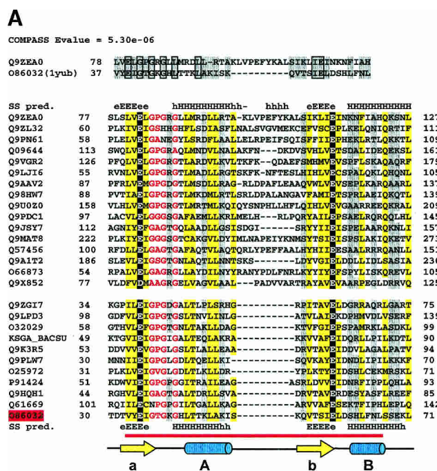
Figure 1. Sequence similarity between the DUF185 and RnaAD families of the PFAM database indicates that DUF185 is a putative methylase domain. (A) Profile–profile alignment, as constructed by COMPASS (shown as the alignment of two representative sequences), and manually refined multiple alignment including representatives from DUF185 (top) and RnaAD (bottom) are illustrated. The TrEMBL identifier and first residue number are shown for each sequence. In the initial COMPASS alignment, matches with positive scores are highlighted in gray, and invariant residues are boxed. In the refined multiple alignment, the uncharged residues (all amino acids except D, E, K, and R) in mostly hydrophobic sites are highlighted in yellow, the nonhydrophobic residues (all amino acids except W, F, Y, M, L, I, and V) at mostly hydrophilic sites are highlighted in light gray, and the small residues (G, P, A, S, C, T, V) at positions occupied by mostly small residues are shown in red letters. The invariant glutamate residues are boxed in black. The identifier of the sequence with known spatial structure in RnaAD (PDB Id 1yub) is highlighted in red. The PHD secondary structure predictions (SS pred.) are shown for this sequence and for the top sequence of the DUF185 alignment. The actual secondary structure of the 1yub fragment is shown below the alignment, with secondary structure elements labeled and colored according to the scheme shown in B. \alpha -Helices and \beta -strands are displayed as arrows and cylinders, respectively. The region covered by the initial COMPASS alignment is shown with a red line below the multiple alignment. (B) A ribbon diagram of the fragment of rRNA methylase (PDB ID 1yub) that was drawn by MOLSCRIPT (Kraulis 1991). N and C termini are labeled. The highlighted region corresponds to the alignment in A; \alpha -helices are colored in blue; \beta -strands are colored in yellow.
